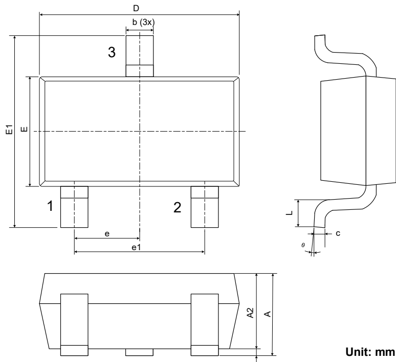
Figure 4. Package Dimension
