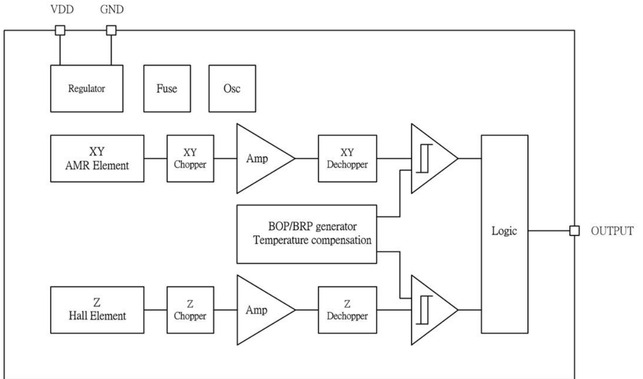
Figure 3. Block Diagram.
