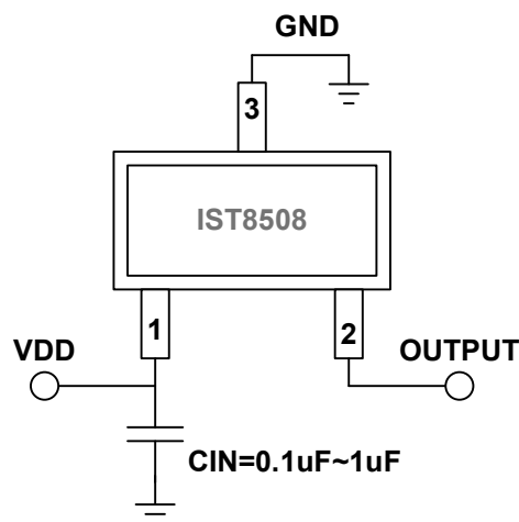
Figure 2. Application circuit
