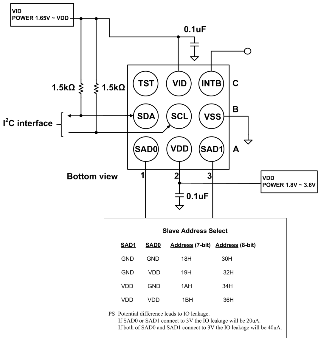
Figure 4. Application Circuit
