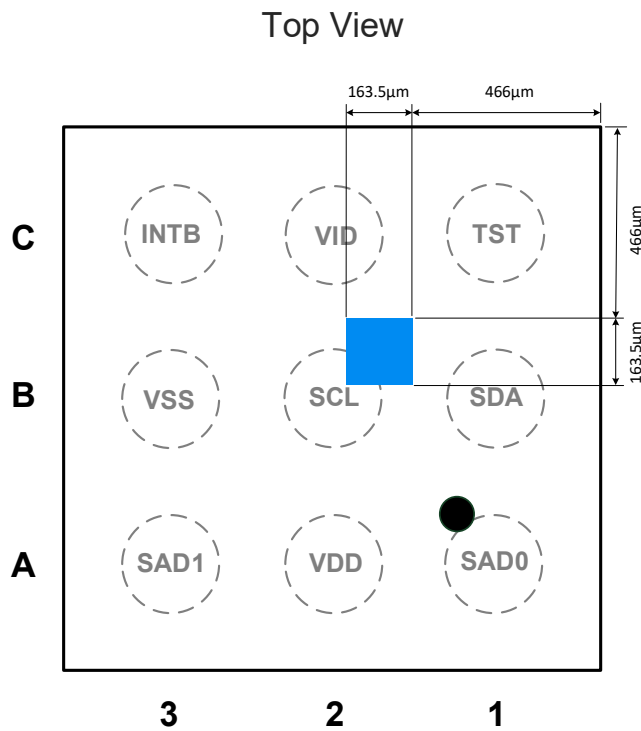
Figure 3. Hall Element Locations
