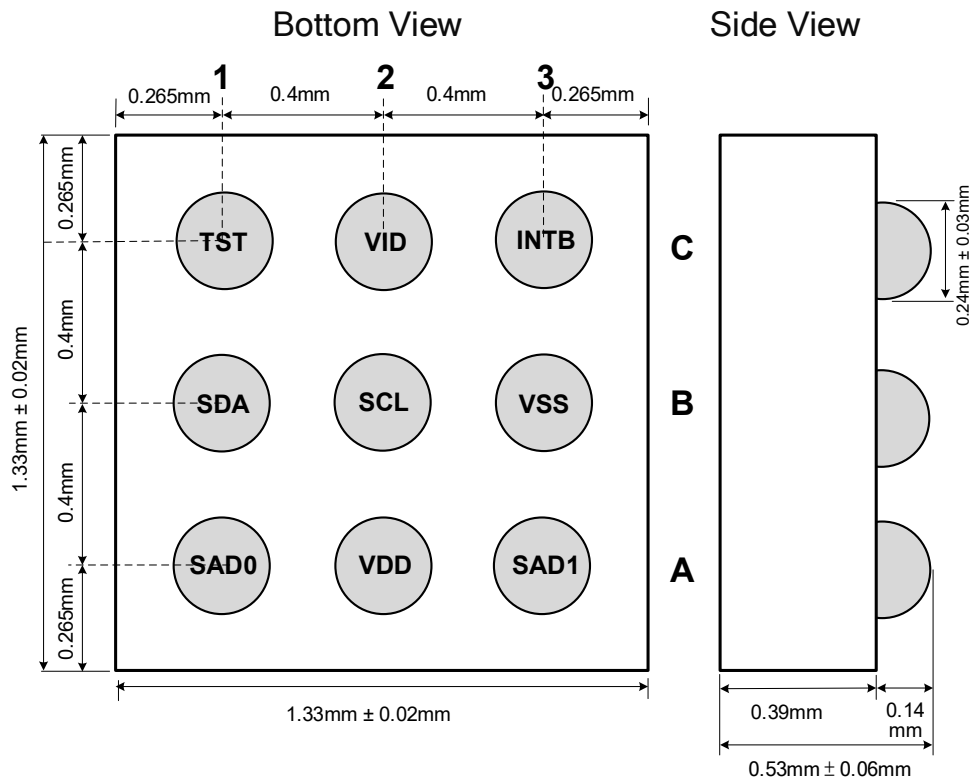
Figure 2. Package Dimensions
